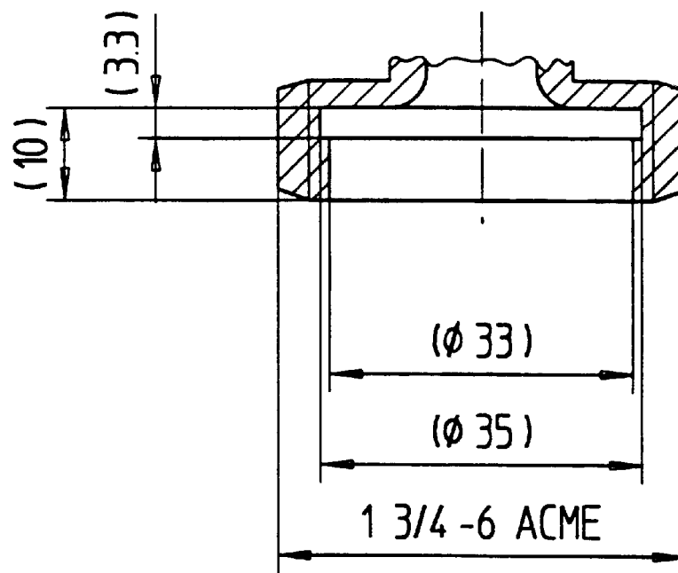
Figure 3 : This filling unit applies only for motor vehicles of categories M2, M3, N2, N3 and M1 having a maximum total mass > 3500 kg. 1/
