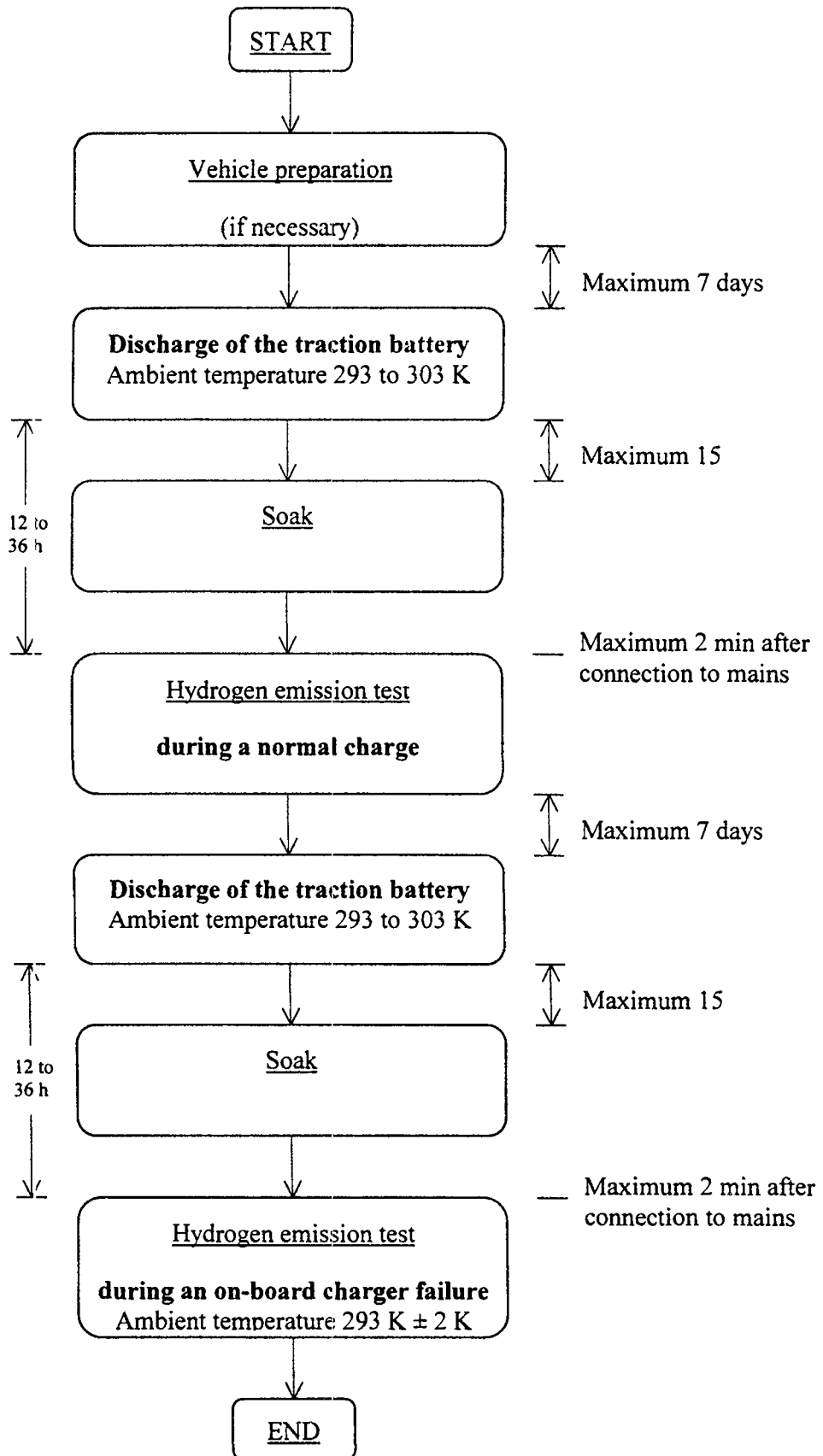
Figure 7.1 Determination of hydrogen emissions during the charge procedures of the traction battery
