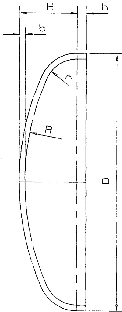
torispherical ends
