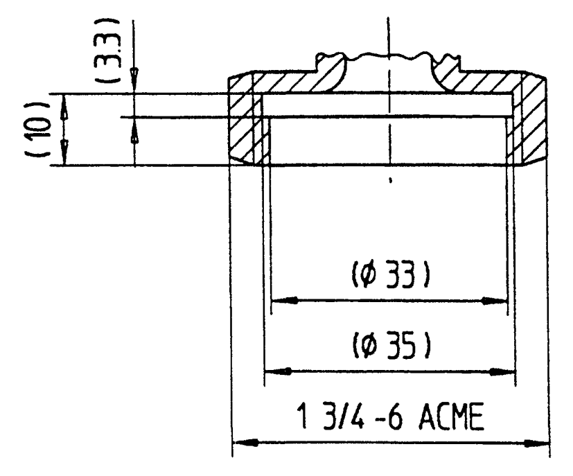
Figure 3: This filling unit applies only for motor vehicles of categories M2, M3, N2, N3 and M1 having a maximum total mass > 3500 kg. 1/
