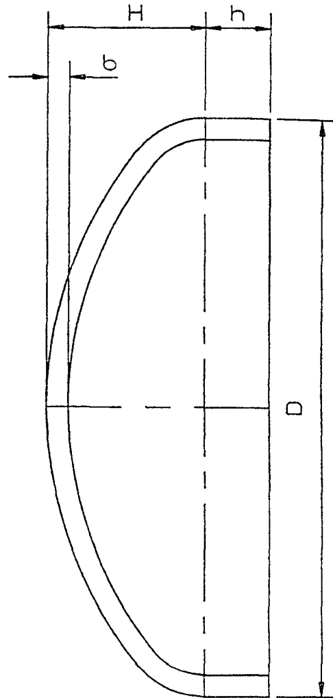
elliptical ends
