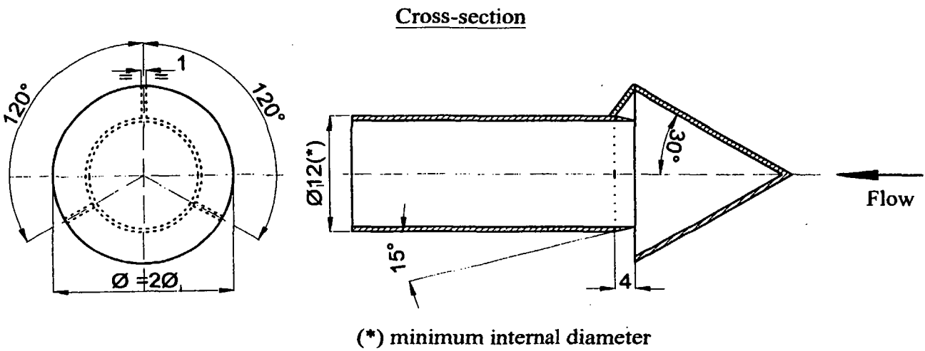
Figure 5/2 Particulate sampling probe configuration
