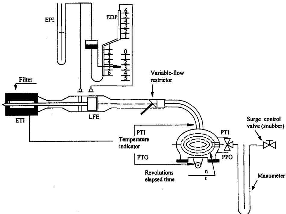
PDP-CVS calibration configuration
